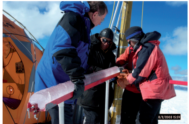
Fig. 3. Ice core that was drilled (in 2003) through the Quelccaya Ice Cap in Peru (5680 m) all the way to the base (Photo by Lonnie G. Thompson).
