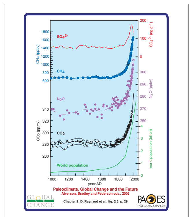
Fig. 4. Anthropogenic increase: records of carbon dioxide, methane, nitrous oxide, and sulfate over the last millennium [1].
