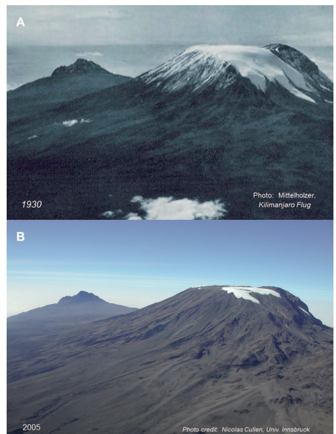
Fig. 5. Kilimanjaro ice cap in (A) 1930 and (B) the year 2005.
