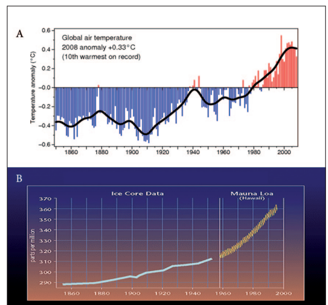
Fig. 2. (A) Temperature as a departure or anomaly from the average, from 1850 to 2008. (B) Ice core record of CO 2 over the same interval of time.
